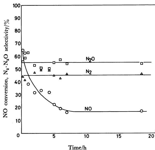
Fig. 1. Reduction of NO over CuHPA supported on DA active carbon.
