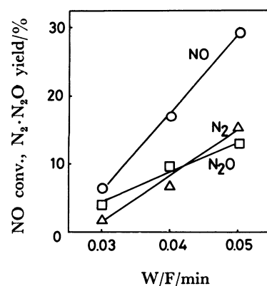
Fig. 2. Dependence of NO conversion on the contact time.
